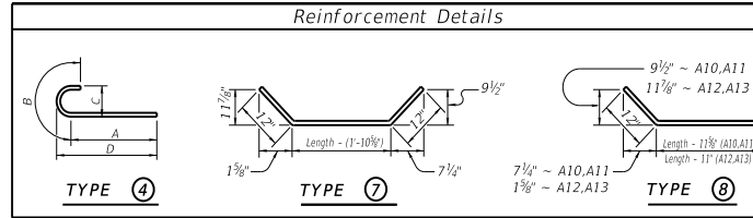
Reinforcement Details
